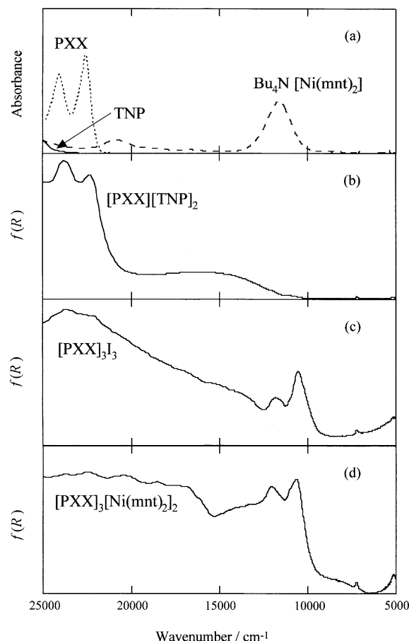
Fig. 3. Vis-NIR spectra of PXX, TNP, and \text{Bu}_4\text{N}[\text{Ni}(\text{mnt})_2] in each chloroform solution (a), diffuse reflectance spectra plotted by the Kubelka-Munk function, f(R) , of [\text{PXX}][\text{TNP}]_2 (b), [\text{PXX}]_3\text{I}_3 (c), and [\text{PXX}]_3[\text{Ni}(\text{mnt})_2]_2 (d).
