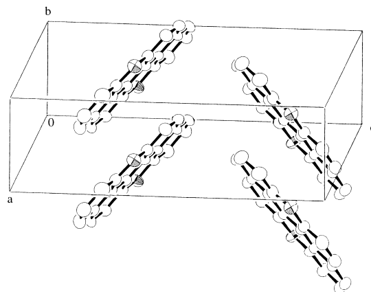
Fig. 1. Crystal structure of PXX.
