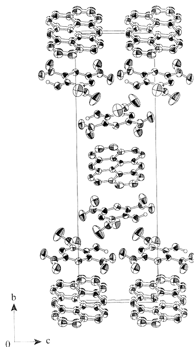
Fig. 4. Crystal structure of [PXX][TNP]_2 .
