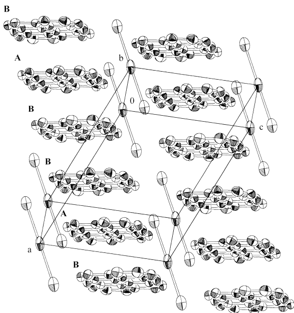
Fig. 5. Crystal structure of [PXX]_3I_3 . A and B are crystallographically independent molecules.
